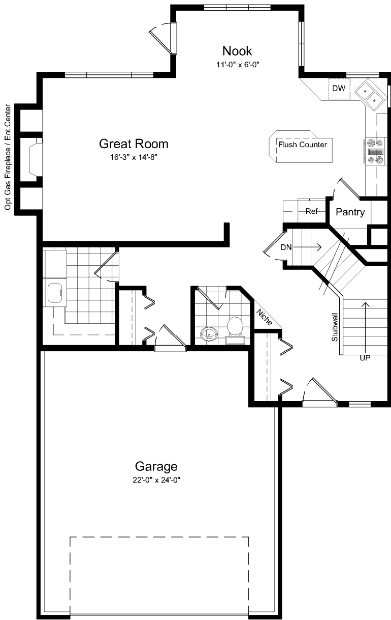
Main Floor 937 Sq. Ft.
